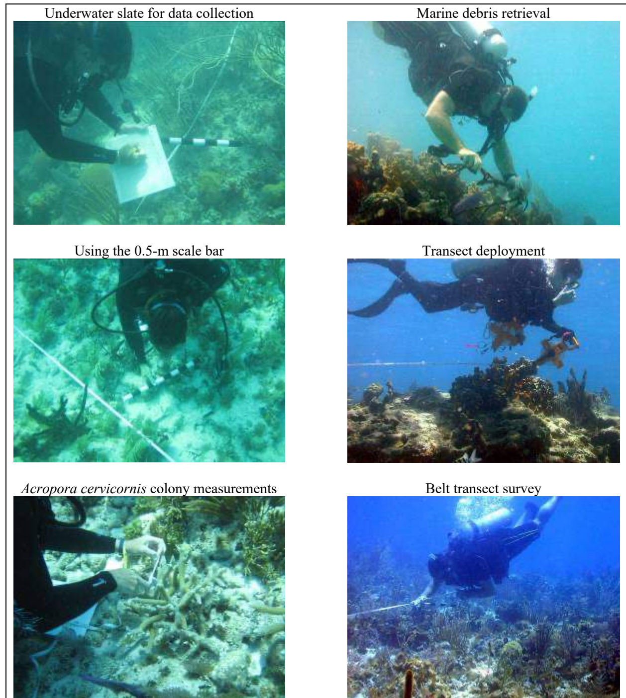
Figure 2-14. Examples of benthic survey methods used by this program to sample Acropora corals, other benthic coral reef organisms, and marine debris.
