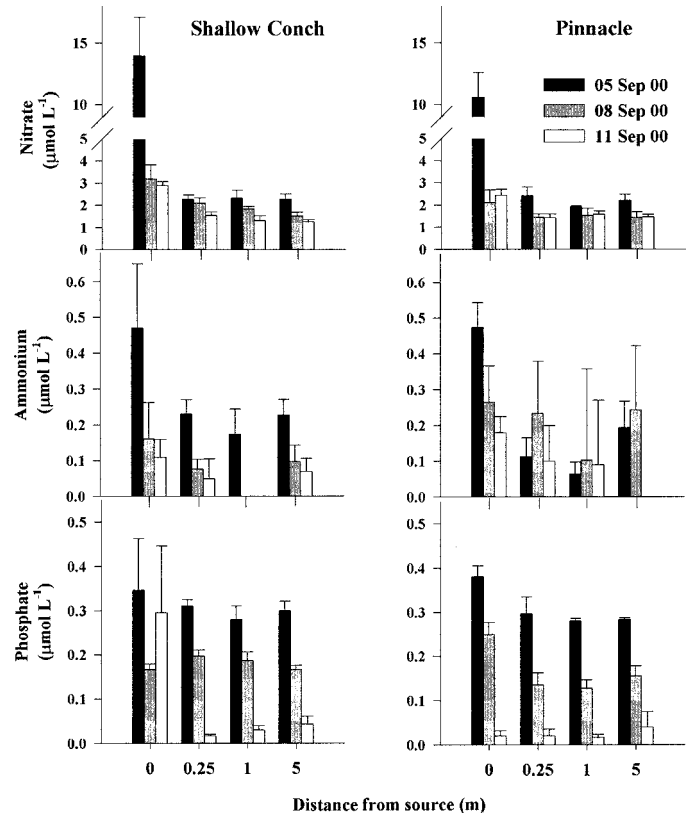
Fig. 3. Experimental nutrient enrichment results (mean \pm 1 SE for nitrate, ammonium, and phosphate, n = 3 ) for water-column samples taken over a 6-d interval beginning 1 h after the deployment of treatments. Different-colored bars represent different sampling dates; distance from source refers to the distance away from the enriched alga.
