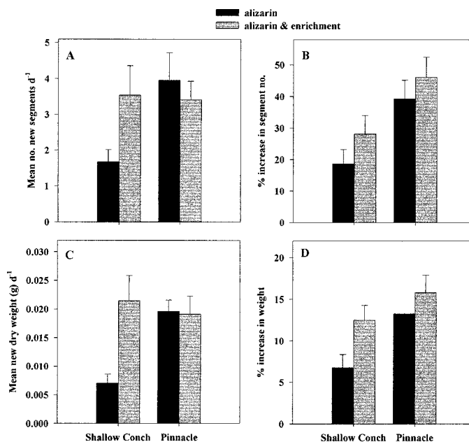
Fig. 5. Mean ( \pm 1 SE, n = 15) of various morphological characteristics for H. tuna at SC and PIN sites in alizarin- and alizarin and nutrient-enriched treatments.
