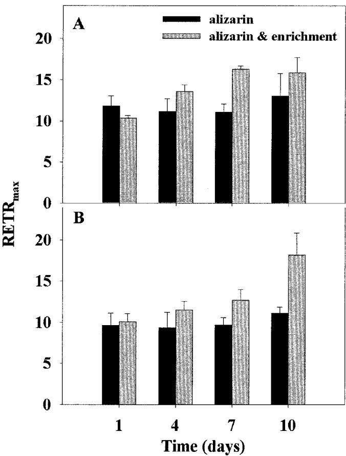
Fig. 10. Changes in RETR max as calculated from rapid light curves for alizarin- and alizarin and nutrient-enriched H. tuna samples from the SC and PIN sites over time.
