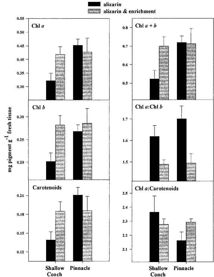
Fig. 8. Photosynthetic pigments (mean \pm 1 SE, n = 12 ) and pigment ratios from H. tuna at the end of the experiment.
