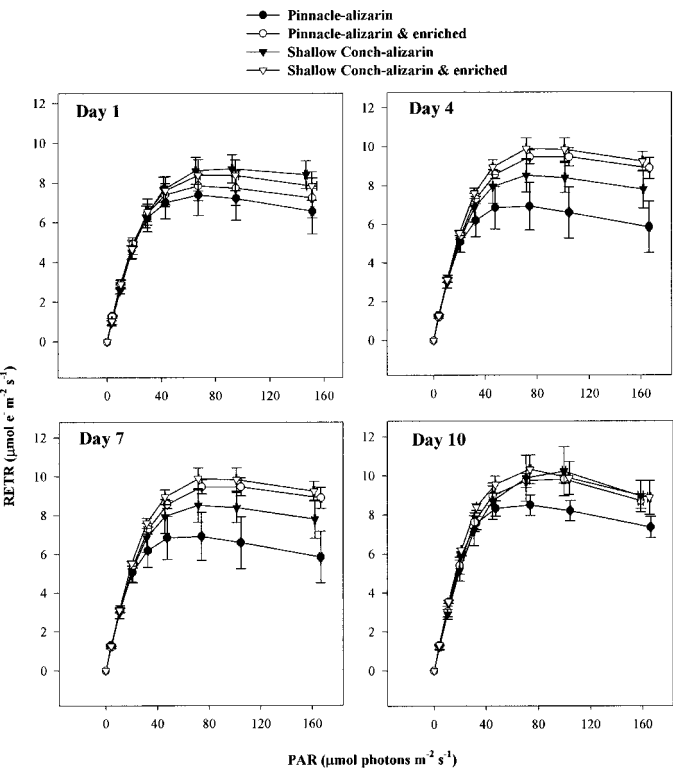
Fig. 9. Rapid light curves generated in the field using a PAM. Each curve represents the mean ( \pm 1 SE, n = 3 ) of three individually sampled H. tuna samples within each treatment and site combination. Curves were run on samples every 3 d during the 10-d nutrient enrichment experiment and began on day 1, immediately after enrichment.
