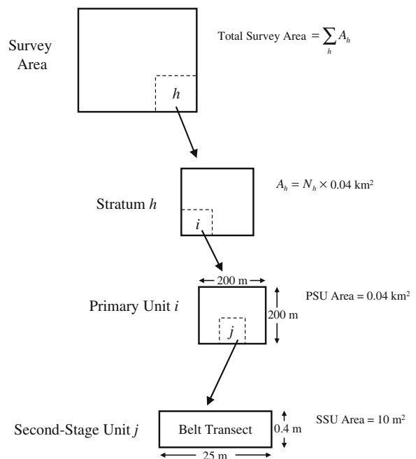
Fig. 2 Conceptual diagram of the survey area, strata, and sample units for a two-stage stratified random survey design. Symbols are defined in Table 1
